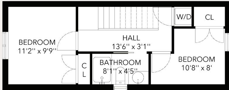
Upper Floor Ceiling Height 8'-0"
