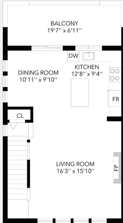
Main Floor Ceiling Height 8' -11"
