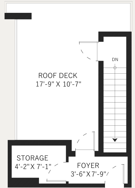
Ceiling Height 8'-0"
