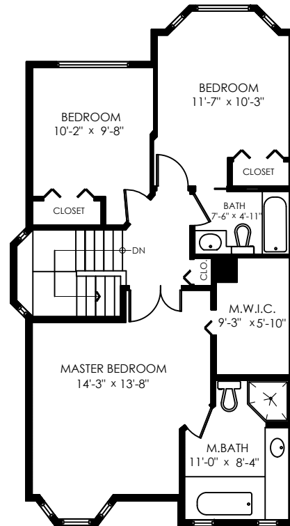
Upper Floor: 825 Sq.Ft. Ceiling Height: 8'-0"
