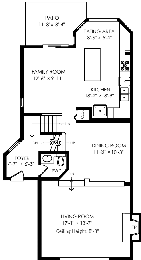
Main Floor: 907 Sq.Ft. Ceiling Height: 8'-0"
